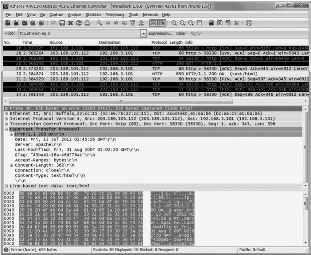
图：Wireshark ( http://www.wireshark.org/ )
